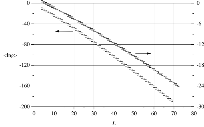
Fig. 1. Averaged logarithm of conductance \langle \ln g \rangle versus size L of the lattice. Calculations are made for for E = -3.5t (circles) and for E = 0.5t (squares). In both cases the population of the samples was 50000. Lines are the fit to Eq. (3). The fitting parameters are d_\phi = 1.144(3) , \xi_l = 0.68(1) , for E = -3.5t and d_\phi = 0.138(3) , \xi_l = 5.13(6) , for E = 0.5t .
